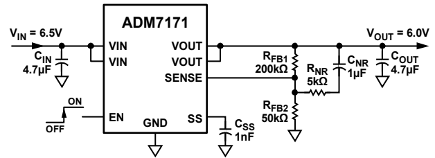
Figure 62. Noise Reduction Modification
