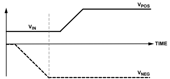
2. V_{NEG} FOLLOWED BY V_{POS} (SEQ = LOW, EN2 = HIGH, EN1 = LOW)
