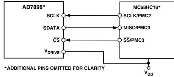
Figure 20. AD7898 to MC68HC16 Interface
