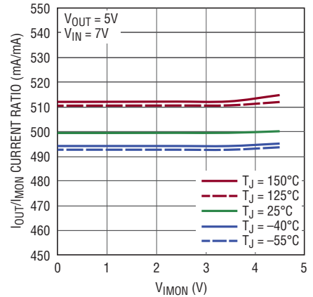
I_{OUT}/I_{MON} Ratio, I_{OUT} = 500\text{mA}
