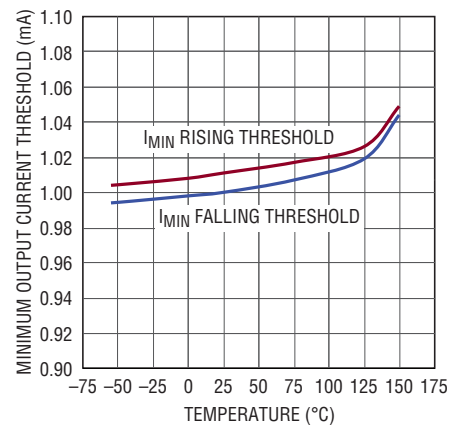
Minimum Output Current Threshold, R_{IMIN} = 1.2\text{M}
