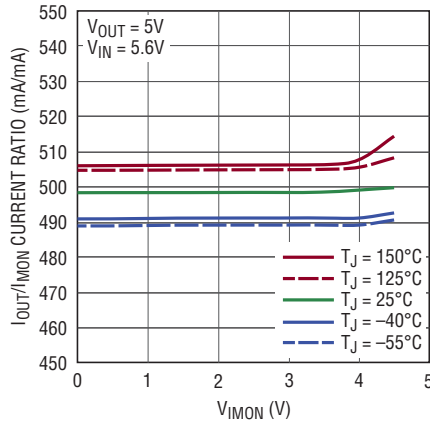
I_{OUT}/I_{MON} Ratio, I_{OUT} = 500\text{mA}
