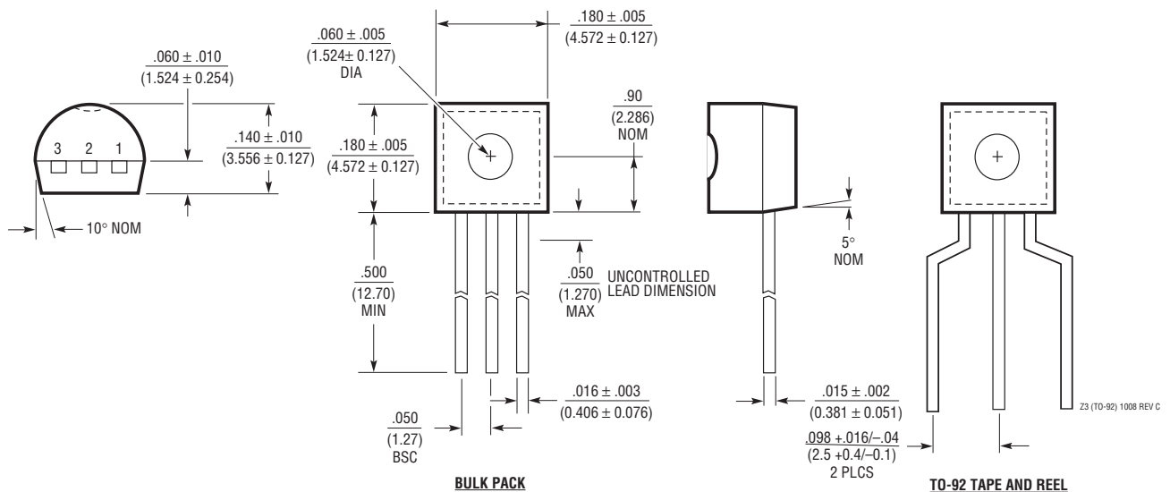
Z Package 3-Lead Plastic TO-92 (Similar to TO-226) (Reference LTC DWG # 05-08-1410 Rev C)
