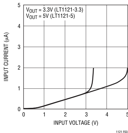
Figure 3. Input Current
