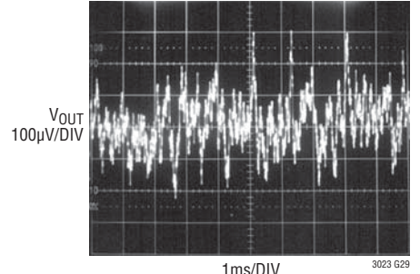
10Hz to 100kHz Output Noise C_{BYP} = 100pF
