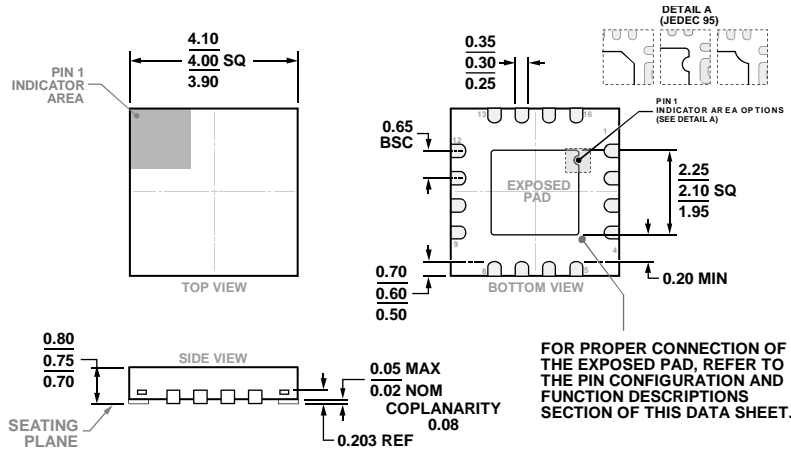
Figure 69. 16-Lead Lead Frame Chip Scale Package [LFCS] 4 mm × 4 mm Body and 0.75 mm Package Height (CP-16-23) Dimensions shown in millimeters
