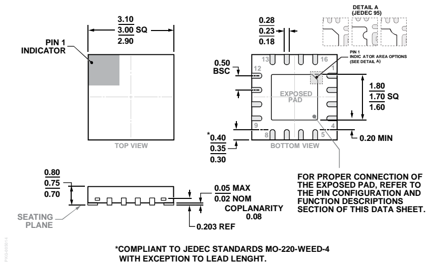
Figure 60. 16-Lead Lead Frame Chip Scale Package [LFCS] 3 mm × 3 mm Body and 0.75 mm Package Height (CP-16-48) Dimensions shown in millimeters
