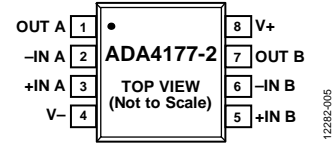
Figure 6. ADA4177-2 8-Lead SOIC Pin Configuration
