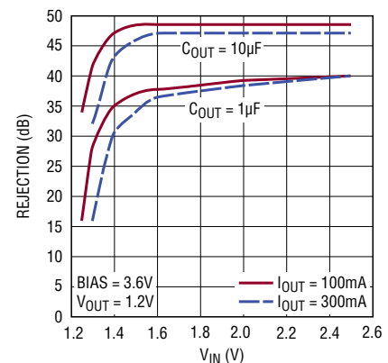
1MHz V IN Supply Rejection
